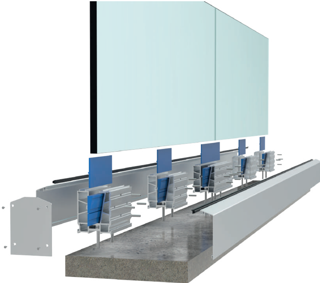
Cam Fitili Glass Rubber
